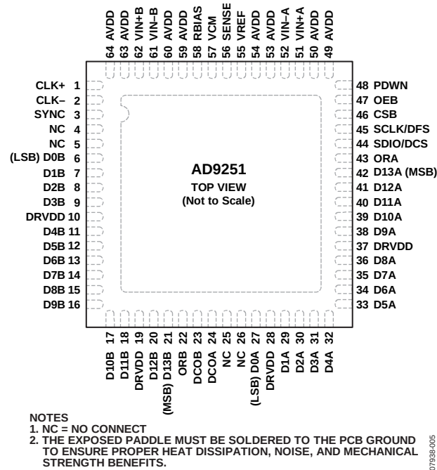
Figure 5. Pin Configuration
